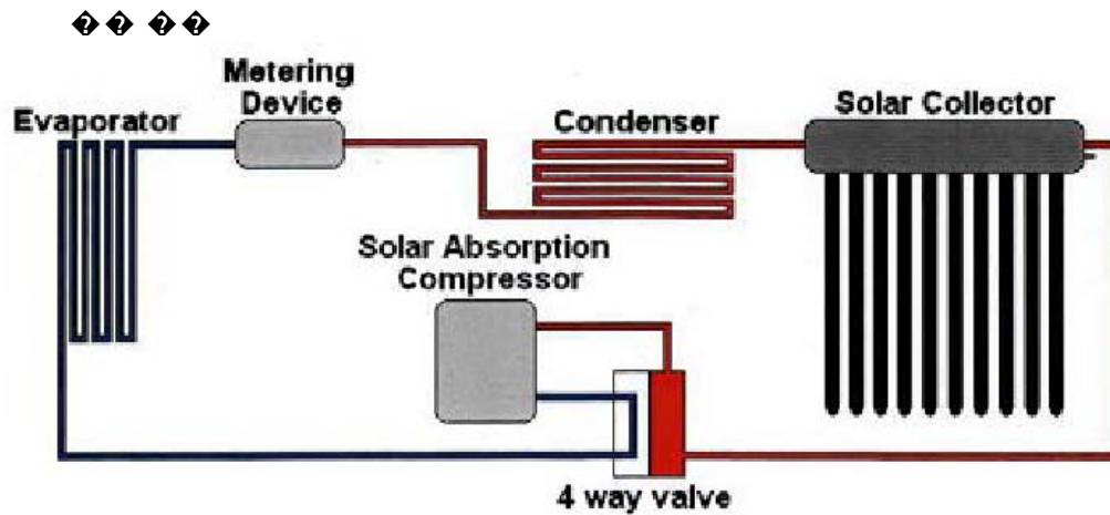
Solar Absorption Diagram
